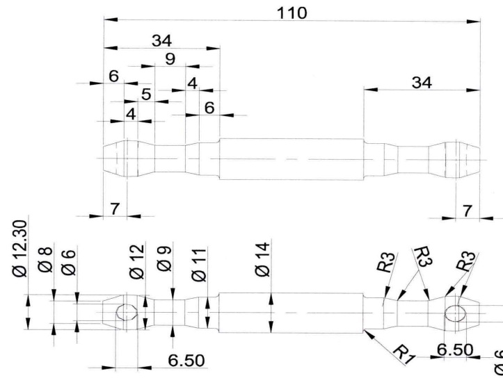
2 COUPLING SHAFT FOR NM 15
