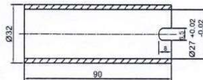
SHAFT SLEEVE
