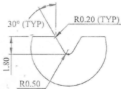
DETAIL-A SCALE 5 : 1
