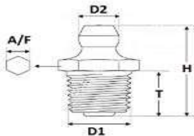
Grease Nipple Size 1/8 BSP-Straight; MOC : SS 304
