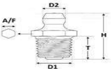
Grease Nipple Size 3/8 BSP-Straight; MOC : SS 304
