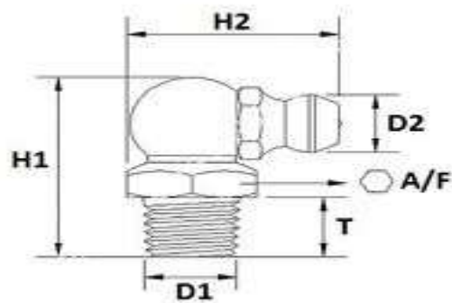
Grease Nipple Size 1/8 BSP-90 Deg; MOC : SS 304
