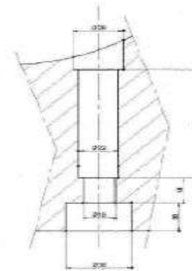
DETAIL-A 4 HOLES AS SHOWN
