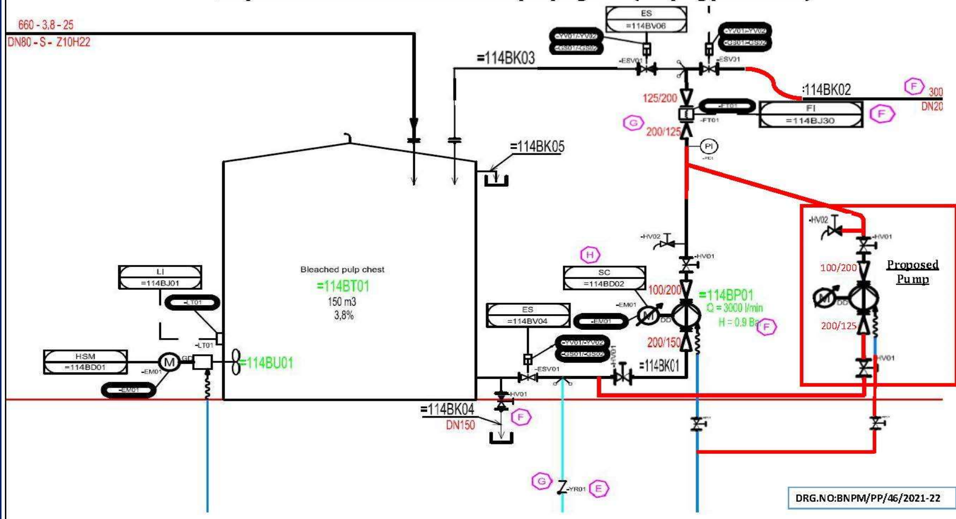
Proposed P & ID for New 150KL Pump Piping PP1 (Pulping plant line 1)
