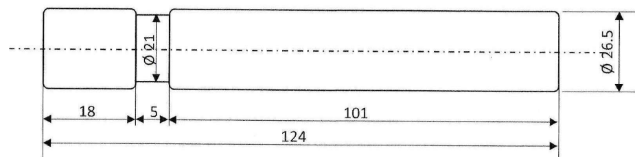
BIVIS Bearing Housing Locking Pin
