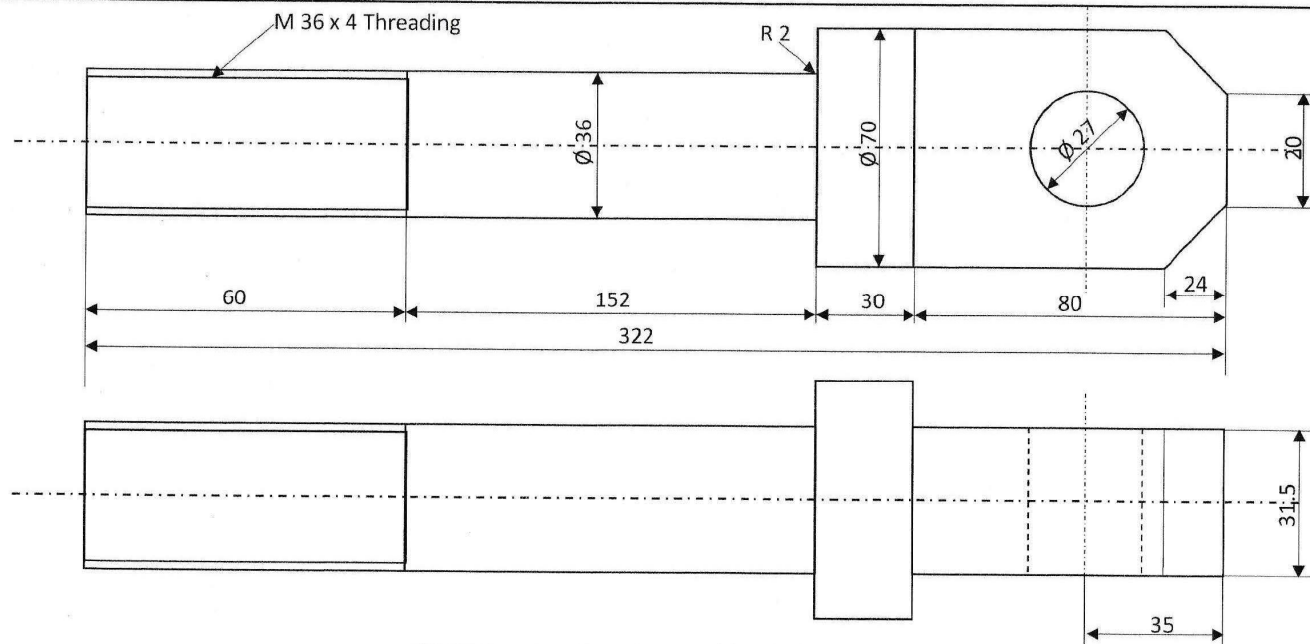
BIVIS Bearing Housing Locking Bolt
