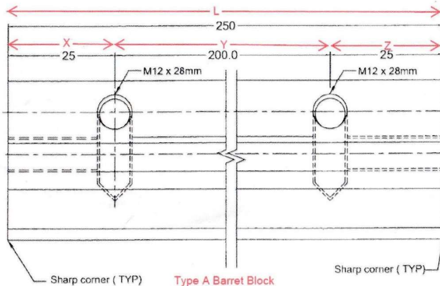
Type A Barret Block
