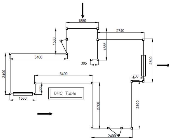
TOP VIEW OF REAM TRANSPORT LAYOUT
