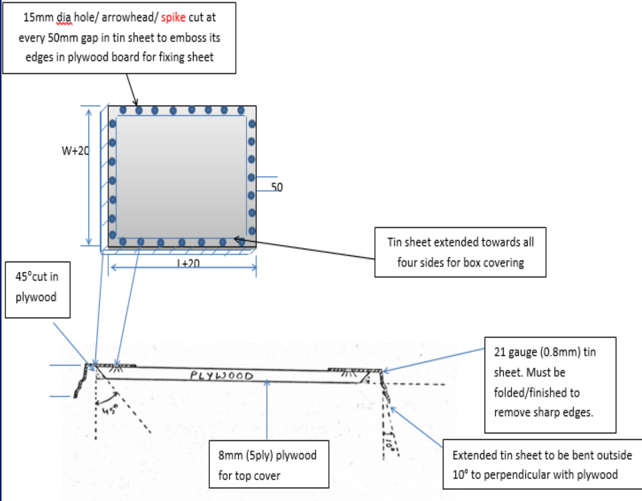
Indicative view for tin sheet fixing
